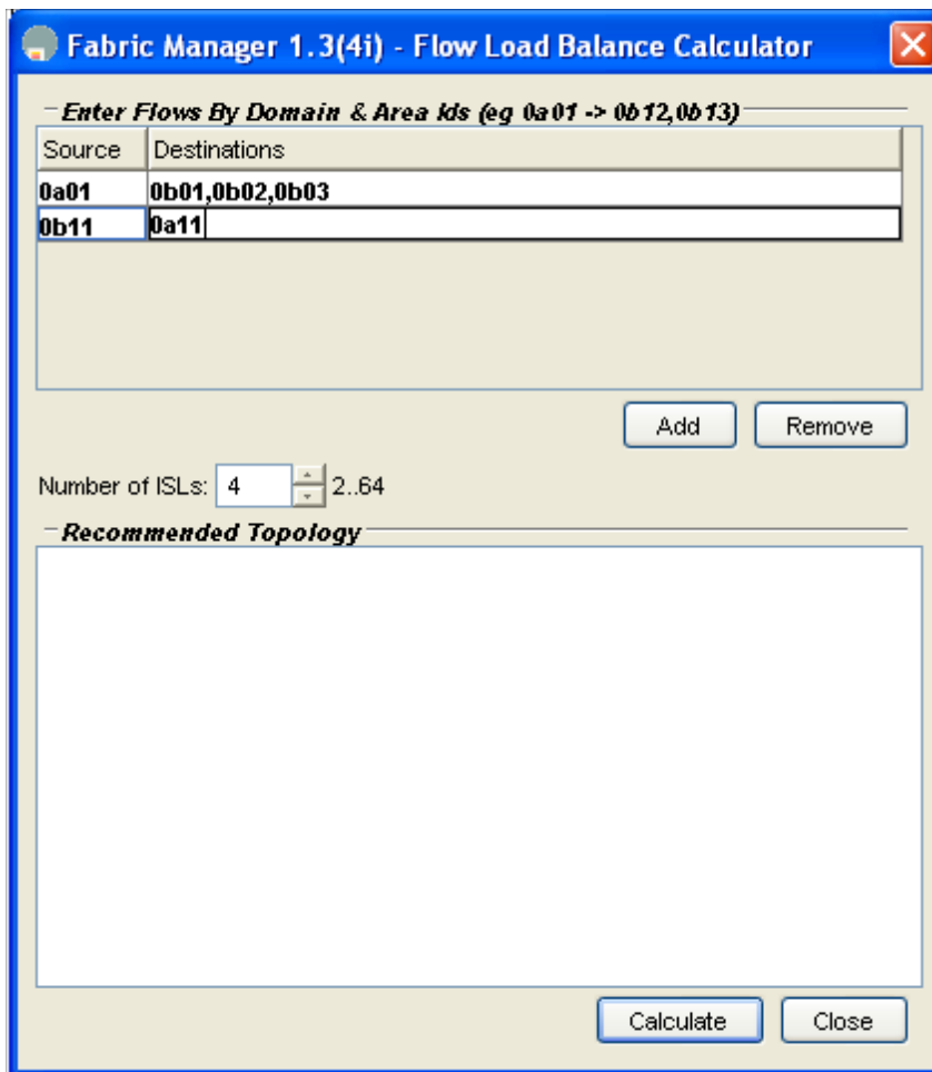
Figure 22-5 Flow Load Balance Calculator - Initial Screen
